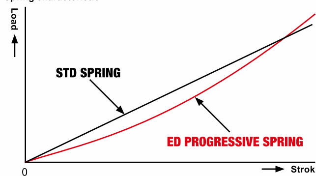
Spring characteristic
